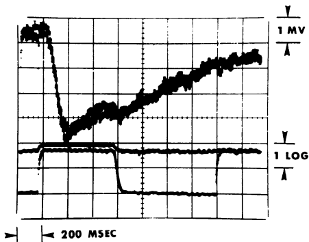
FIG. 5. The autonomy of the receptor response is illustrated by these two superimposed records. One record was obtained with spot illumination flashed on the receptor with the retina in the dark. For the second record, an annulus (of 250- \mu radius) around the electrode was maintained on (elevated base line in stimulus recording), and then the receptor was illuminated with the same spot as in the first case. The two records are almost identical, indicating that under these conditions illumination of the surround does not affect the response of the receptor.
