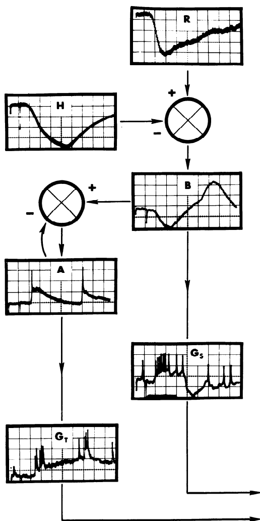
FIG. 12. Summary diagram of synaptic organization of the retina. Transformations taking place in each plexiform layer are represented here by summing junctions. At the outer plexiform layer the direct input to the bipolar cell from the receptor is modified by input from the horizontal cells. At the inner plexiform layer the bipolar cell drives some ganglion cells directly. These ganglion cells generate a sustained response to central illumination; and thus these cells follow the slow, sustained changes in the bipolar cells' response. Bipolar cells also drive amacrine cells, and the diagram suggests that it is the amacrine-to-bipolar feedback synapse that converts the sustained bipolar response to a transient polarization in the amacrine cell. These amacrine cells then drive ganglion cells which, following the amacrine cell input, respond transiently.
