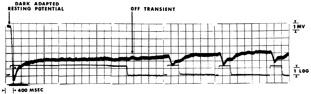
FIG. 4. Time course of response for a receptor. Response of the dark-adapted receptor begins with a large initial transient which decays to a steady hyperpolarization that is graded with the intensity of stimulus. When the stimulus is terminated, the response begins to decay to the original resting potential, with a surprisingly small off-transient. Additional stimuli of the same intensity, presented before the cell fully dark adapts, evoke responses with small initial transients that decay to the same steady hyperpolarized level that is independent of the state of adaptation.
