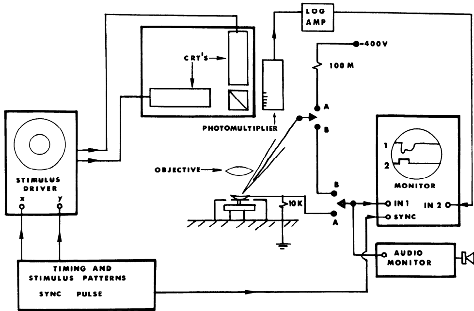
FIG. 1. Apparatus for stimulation, recording, and staining. Patterns generated on the faces of the two cathode-ray tubes (CRTs) are combined in the beam-splitting prism and focused on the retina. The other output from the prism illuminates the face of a photomultiplier. Output from the photomultiplier is linear with intensity throughout the range used here. This linear signal is logarithmically compressed and appears as the lower trace, 2, in all recordings presented in the paper. One log unit of intensity is represented by one vertical division. The electrode is coupled, either to the d-c recording amplifier and then to the oscilloscope (B) or to the negative 400-v staining potential (A), by the relay system. When the stain is ejected, current flows through the electrode, the preparation, and the 10-kilohm resistor to ground. The potential produced by the staining current across the 10-kilohm resistor is monitored by the audio amplifier. Timing is controlled so that the oscilloscope sweep begins in all recordings 200 msec before the retina is stimulated. In this way, timing for all recordings can be estimated from the initial segment of the trace.
