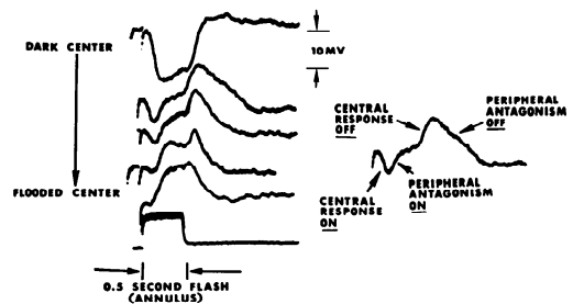
FIG. 10. Latency difference between the center and surround response of the bipolar cell. The series of responses shown here was elicited by annular stimulation sufficiently bright to yield considerable scatter into the center of the field. Maintained intensity at the center of the field was gradually increased to reduce the effect of scatter from the flashing annulus. The effective ratio of stimulation of center and surround is thereby gradually shifted to favor the surround. However, for any ratio of central and surround stimulation, the central response always occurs first. This is shown by the transient hyperpolarization in all traces except the lowermost trace. No center response is observed in the lowermost trace because the maintained central illumination was saturating.
