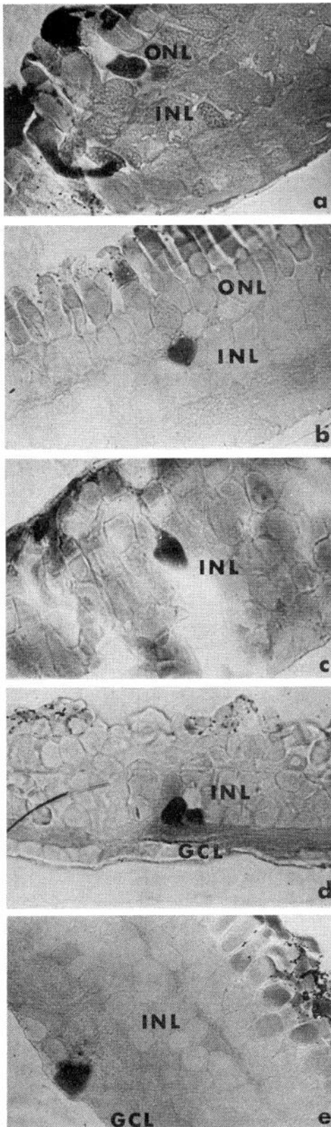
FIG. 2. Intracellularly stained cells such as these were used to establish the identity of recorded responses. The receptor cells (a) always show stain in the inner segment or nucleus. The horizontal cell (b) shown here is located along the outer margin of the inner nuclear layer and has a flattened distal surface where processes extend into the plexiform layer. Bipolar cells (c) are located in the outer half of the inner nuclear layer. The bipolar cell morphology of an elongated cell body is represented in this section, although the overall preservation of this retina is poor. Amacrine cells (d) stain typically along the inner margin of the inner nuclear layer. In the example shown here there is a faint blue staining of an adjacent cell, probably due to leakage of the stain. The deeply stained cell is almost certainly the cell recorded from, but in any case the layering of the stain along the inner margin of the inner nuclear layer is unequivocal. Ganglion cells (e) are easily identified in the single row of cells proximal to the inner plexiform layer. ONL, outer nuclear layer; INL, inner nuclear layer; GCL, ganglion cell layer.
