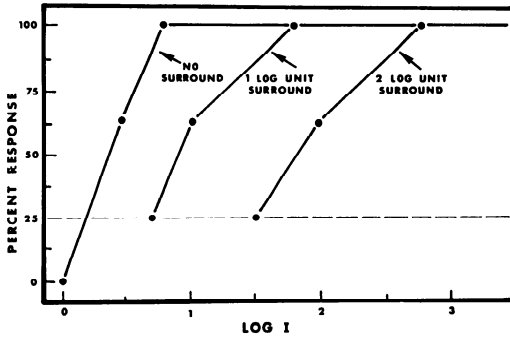
FIG. 8. Intensity-response relations for the bipolar cell. The bipolar response is determined by two parameters: energy falling in the center and energy falling in the periphery of the unit's receptive field. The three curves plotted here for a typical bipolar cell show how the polarization increases with increasing central illumination for three different values of peripheral illumination. The level of saturation is the same in all cases, but the dynamic range for the response is shifted along the intensity axis as the surround illumination is increased. Dotted line above the resting potential indicates that in this cell the surround could not turn off the polarization completely.
