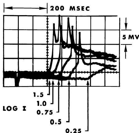
FIG. 11. Latencies of the amacrine response as a function of stimulus intensity. Five responses obtained with different intensities of stimulation were superimposed. Recordings show how the latency decreases with increasing stimulus intensity although the form of the response—one or two spikes superimposed on a transient slow potential—remains relatively unchanged.
