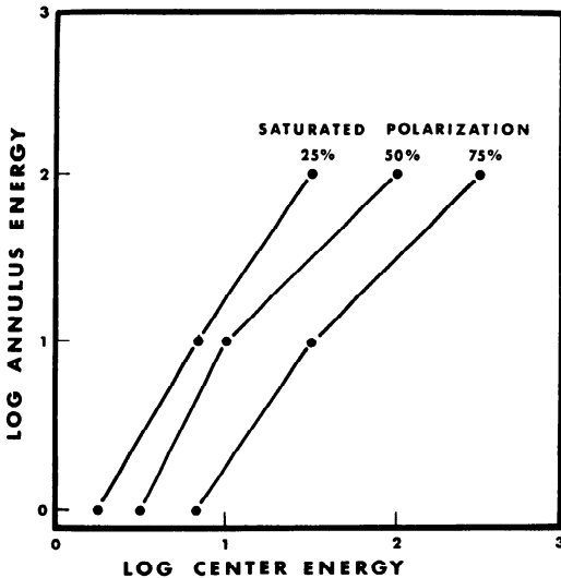
FIG. 9. Contrast detection properties of the bipolar cell. The abscissa and ordinate in this figure represent the total energies of stimulation falling in the center and periphery of receptive field for the bipolar cell. Each curve represents the relative quantities of each energy required to keep the polarization in the bipolar cell fixed. These curves indicate that the polarization is maintained by a fixed ratio of energy falling at the center versus the surround of the field. The curves suggest that the difference function is computed before saturation of either component. If this were not the case it would be impossible to increase the polarization of the unit after it had once been saturated.
