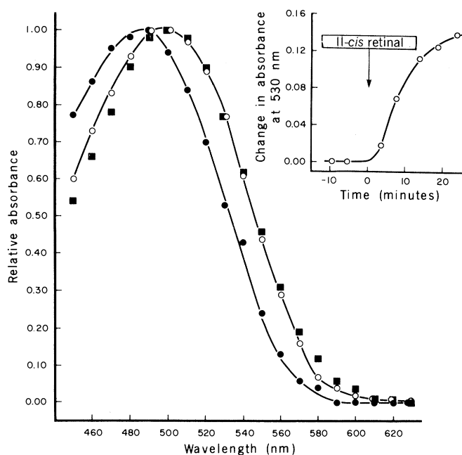
Fig. 2. Normalized difference spectra obtained in the presence of hydroxylamine. In one experiment (○), a dark-adapted isolated retina was exhaustively bleached with Wratten 58-filtered light; the 5-minute bleaching exposure eliminated at least 97 percent of the rhodopsin originally present. Eighteen minutes after the offset of the bleaching light, 11- cis retinal (1.7 \mu mole), suspended in 0.11 ml of ethanol-aspartate Ringer solution (1 : 5 by volume), was gently applied dropwise to the retina. Shown in the inset is the time course of changes in absorbance at 530 nm following the application of the 11- cis retinal. Approximately 26 minutes after the application of the 11- cis retinal, the preparation received 0.10 ml of 0.70M hydroxylamine (pH 6.0), applied dropwise to the upper surface of the retina. Beginning 12 minutes after the treatment with hydroxylamine, the retina was subjected to a second 5-minute bleaching exposure; the open circles represent normalized differences in absorbance which resulted from the second intense illumination. In a second experiment (●), a dark-adapted isolated retina was similarly treated, except that 9- cis retinal (1.7 \mu mole), suspended in 0.11 ml of ethanol-aspartate Ringer solution (1 : 5 by volume), was applied to the retina after the first bleaching exposure; as above, the filled circles represent normalized differences in absorbance which resulted from a second 5-minute bleach carried out in the presence of hydroxylamine. In a third experiment (■), a dark-adapted isolated retina was treated with hydroxylamine and subsequently bleached for 5 minutes; the filled squares represent the normalized difference spectrum obtained as a result of this single exposure. The peak absolute values of absorbance for the difference spectra illustrated are (○) 0.161 (at 500 nm), (●) 0.094 (at 490 nm), and (■) 0.285 (at 500 nm).
